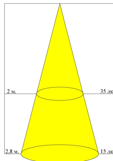
Geniled EVO E27 G45 5W (4200K)
