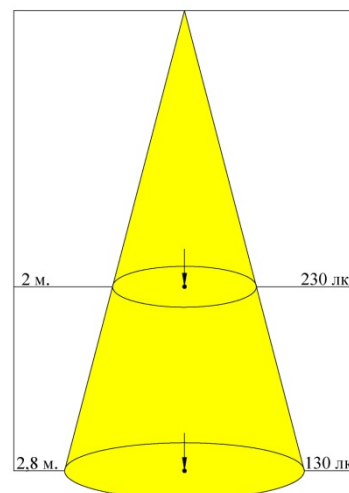
KCCGeniled G13 T8 25W(4200K)
